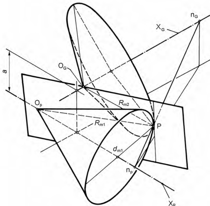
Figure A.2 — Schematic of hypoid gear
