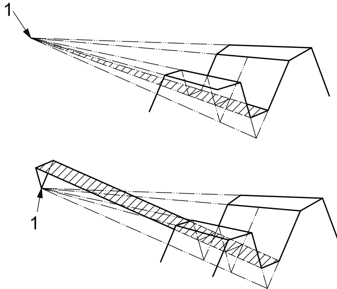
Figure 9 — Root line tilt
