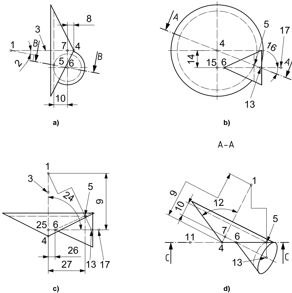
Figure 14 — Hypoid geometry
